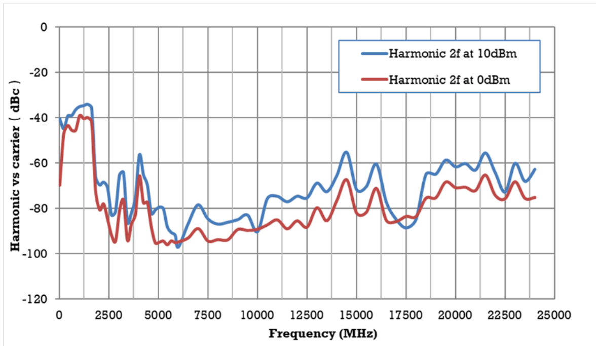
Second harmonic versus carrier frequency at level 0 dBm&amp;10 dBm
