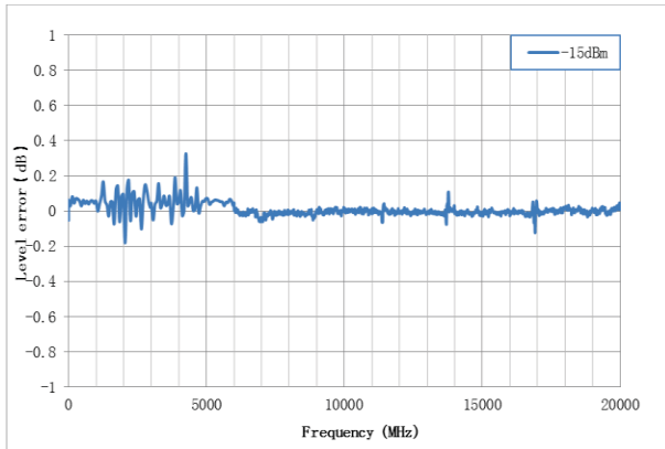
Measured level error frequency, Level = - 15 dBm
