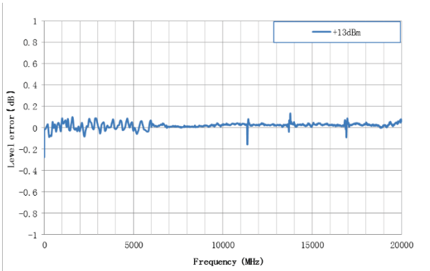
Measured level error versus frequency, Level = + 13 dBm
