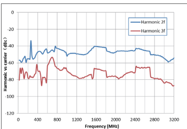
Measured harmonics versus carrier frequency at level \le +13 \text{ dBm}
