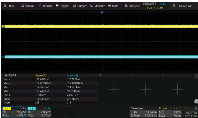
Low noise floor: 125 \mu Vrms at 1 GHz bandwidth
