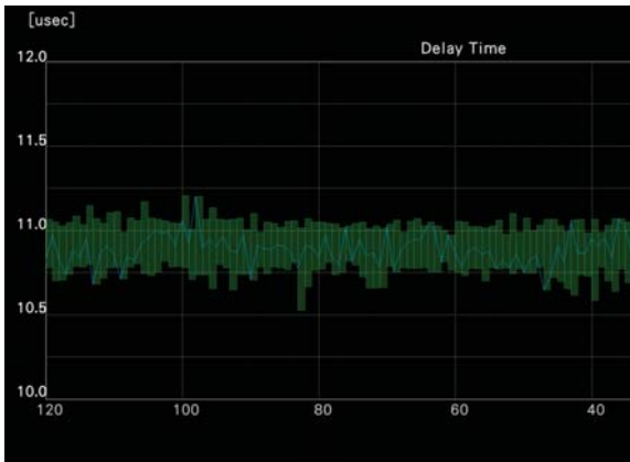
Time difference per second display as a graph over time
