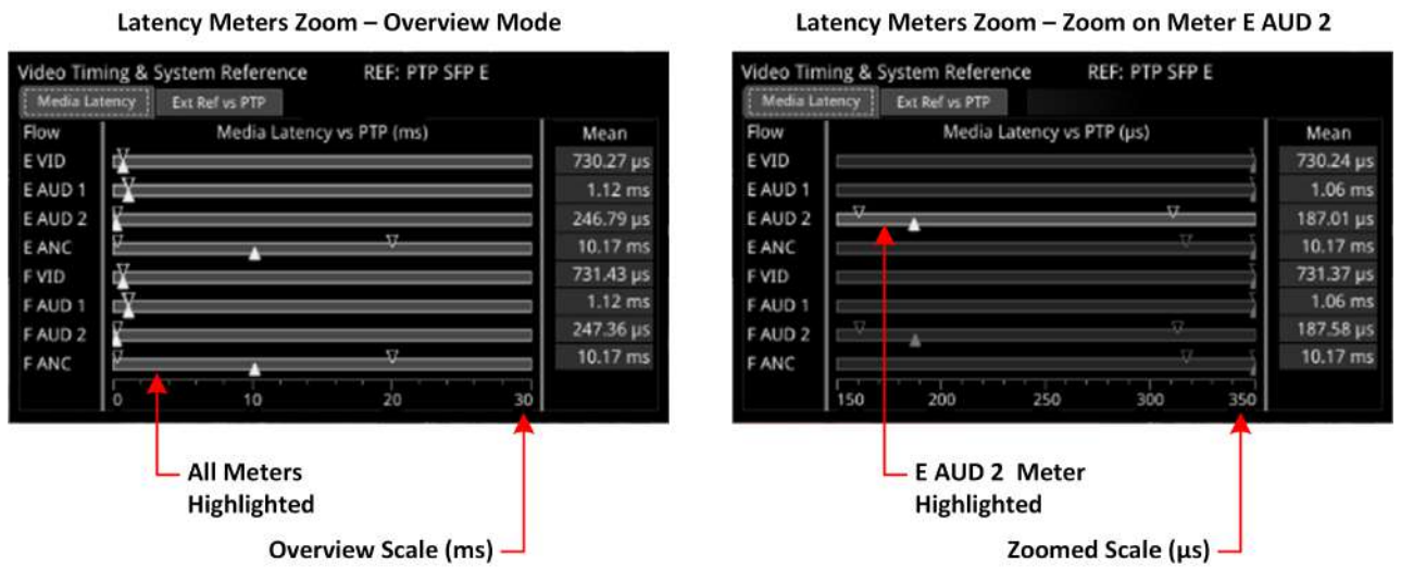
Figure 4-33: Media Latency Tab of the Video Timing & System Reference Instrument (ST 2110 IP Input)
