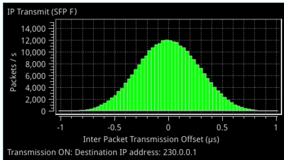
Figure 6-29: 2022-6 Transmit (SFP F)
