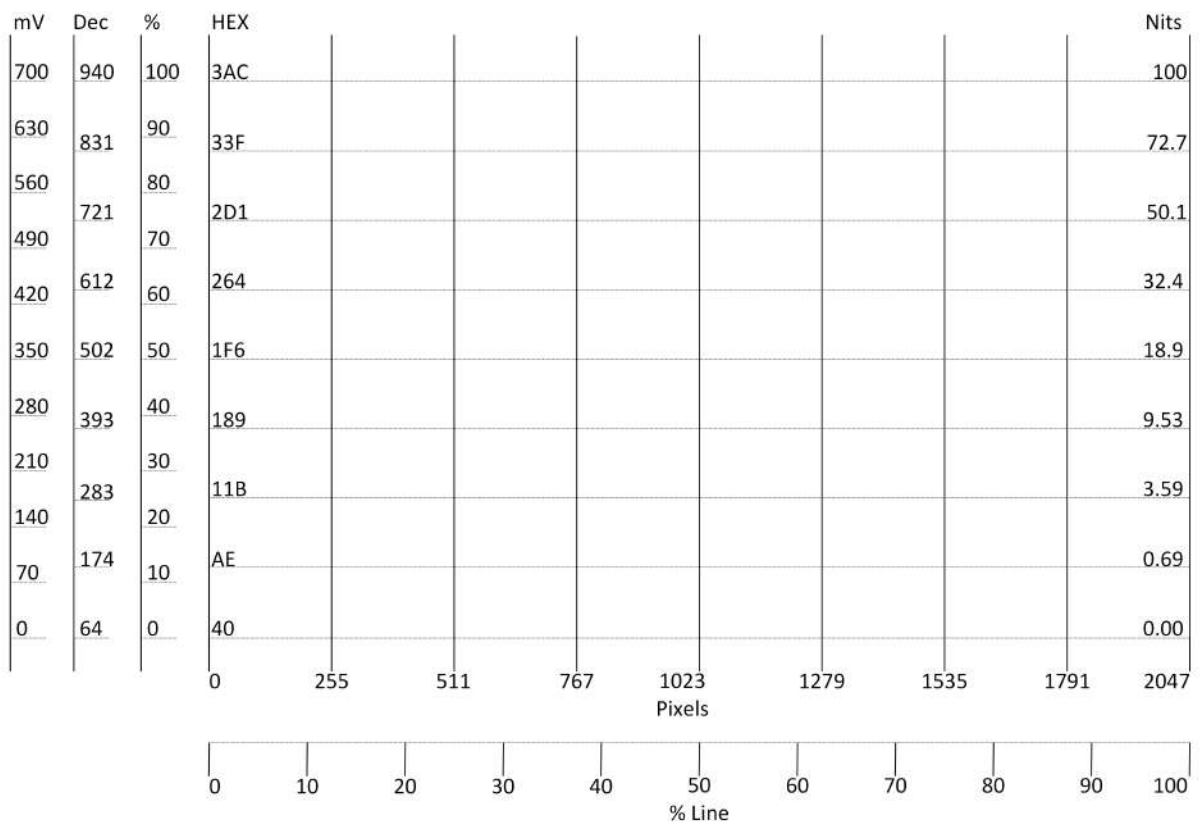
Figure 9-13: Schematic of Waveform Scales (Overlay Mode; SDR 2048 x 1080; Narrow Range, Full Screen Size)
