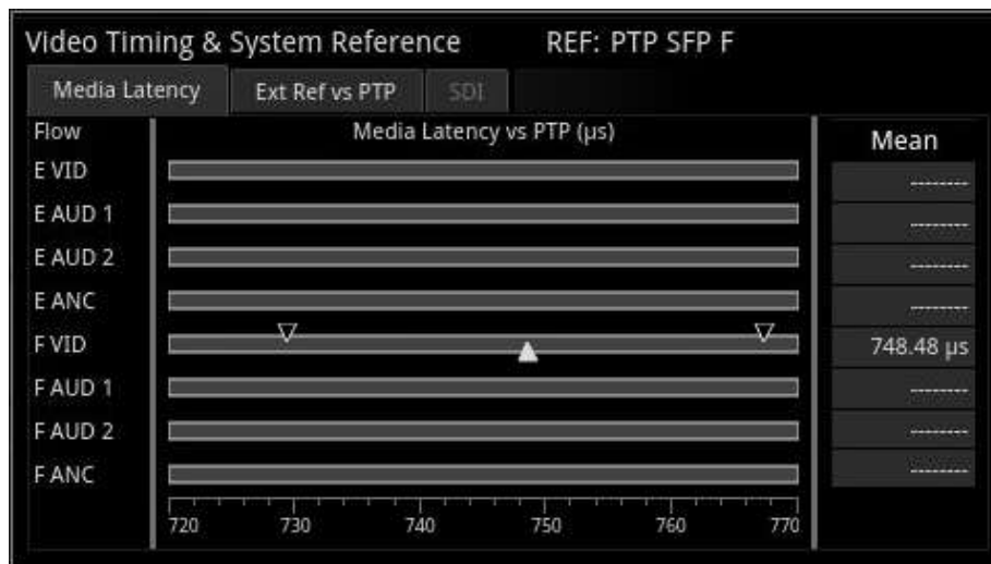
Figure 4-32: Media Latency Tab of the Video Timing & System Reference Instrument (ST 2110 IP Input)
