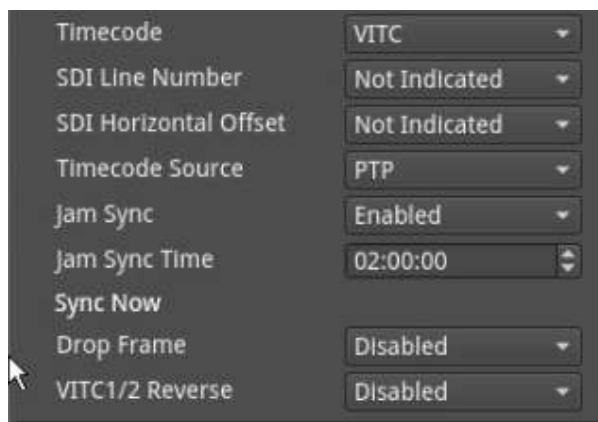
Figure 6-16: ATC Timecode Parameters in the Generator Options Menu (ST 2110 IP Output)
