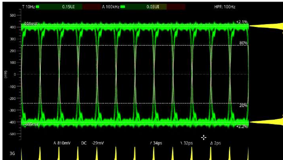
Figure 13-2: 3G-SDI Eye Pattern Set to Display 12 Eyes (Using Green Display Color) (Optional SDI Input)
