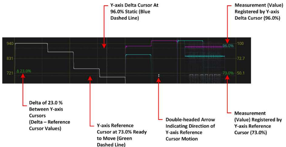
Figure 9-24: Waveform Measurement Y-axis Cursors (Independent Configuration)
