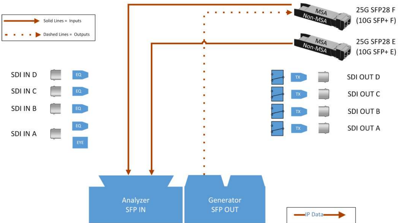
Figure 4-2: IP Input/Output Modules to Analyzer / Generator Circuitry (ST 2022-6 IP Input)
