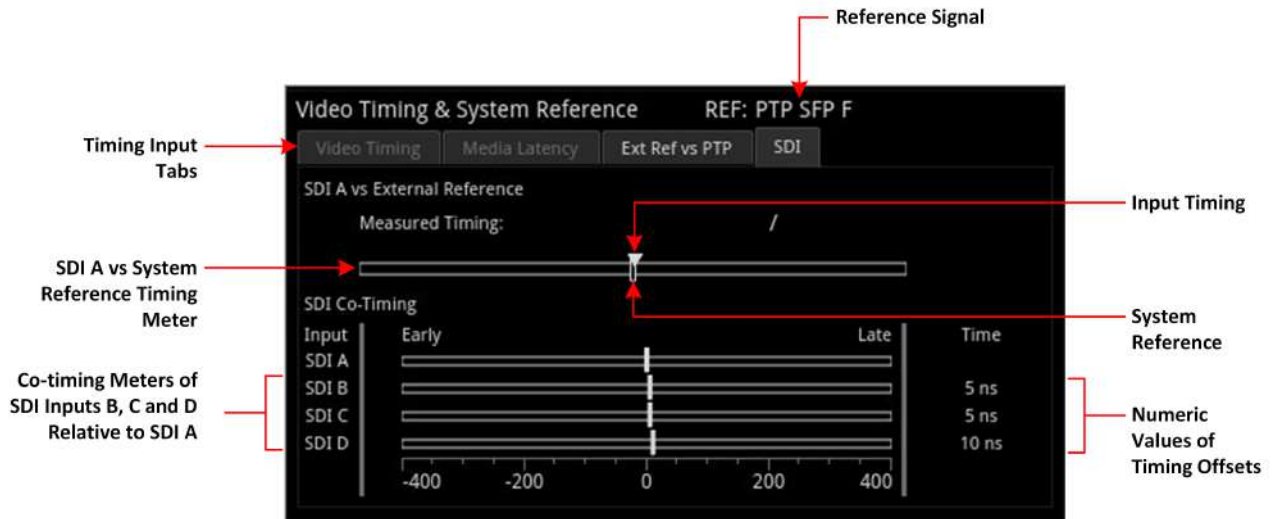
Figure 5-15: Video Timing & System Reference Instrument (SDI Input)
