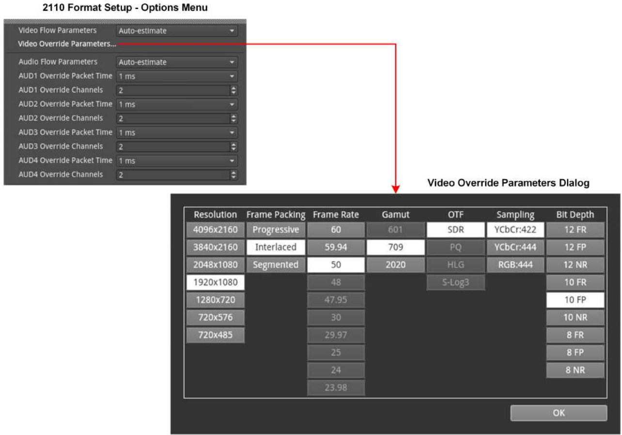
Figure 4-44: Analyzer - 2110 Format Setup Instrument - Options Menu and Video Override Parameters Dialog
