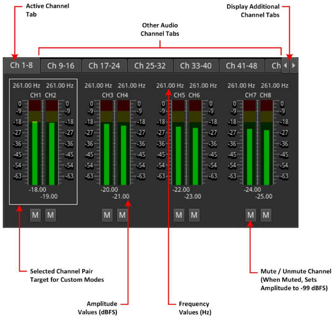
Figure 6-27: Audio Generator Configuration Dialog - Audio Channel Selection Panel
