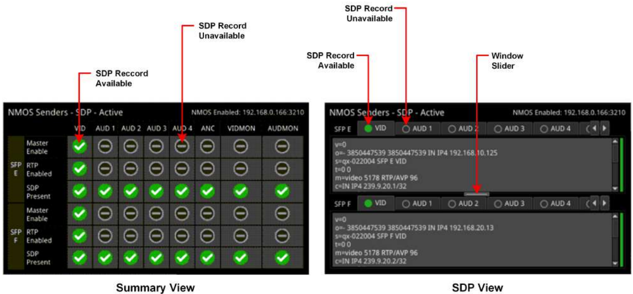
Figure 4-22: NMOS Senders - SDP Instrument (Single Interface, 1/16 Screen Size) (ST 2110 IP Inputs)
