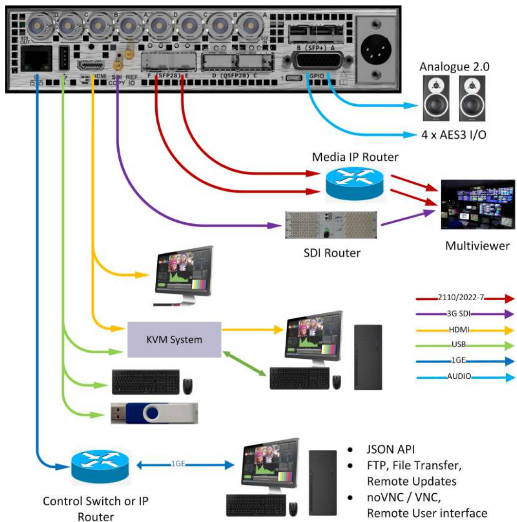
Figure 3-31: Remote Connectivity Overview
