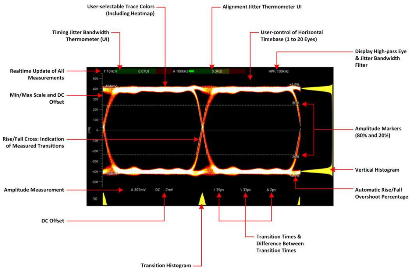
Figure 13-1: Standard SDI Eye Pattern Display (3G) with 100 kHz Jitter Filter (Optional SDI Input)
