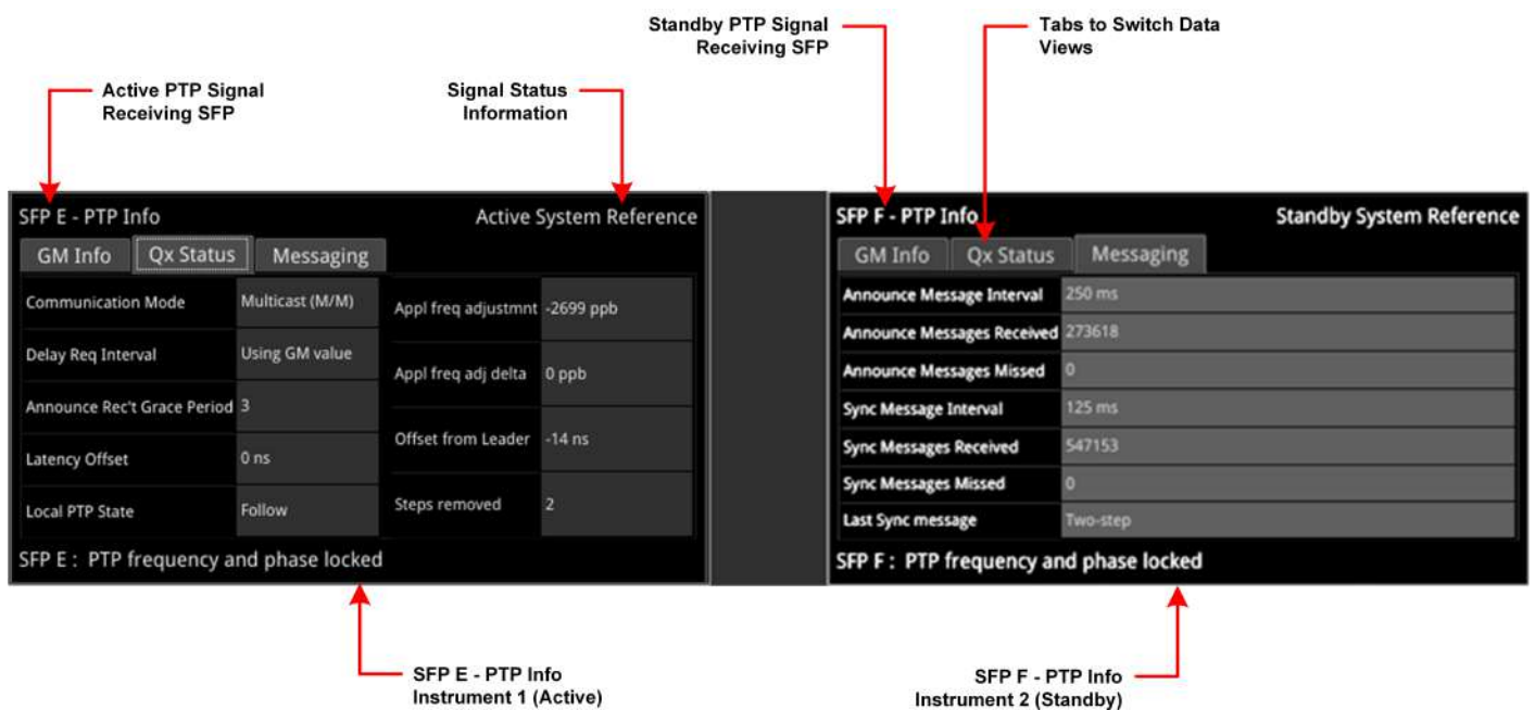
Figure 4-28: Dual SFP E and F - PTP Info Instruments (ST 2110 IP Input)
