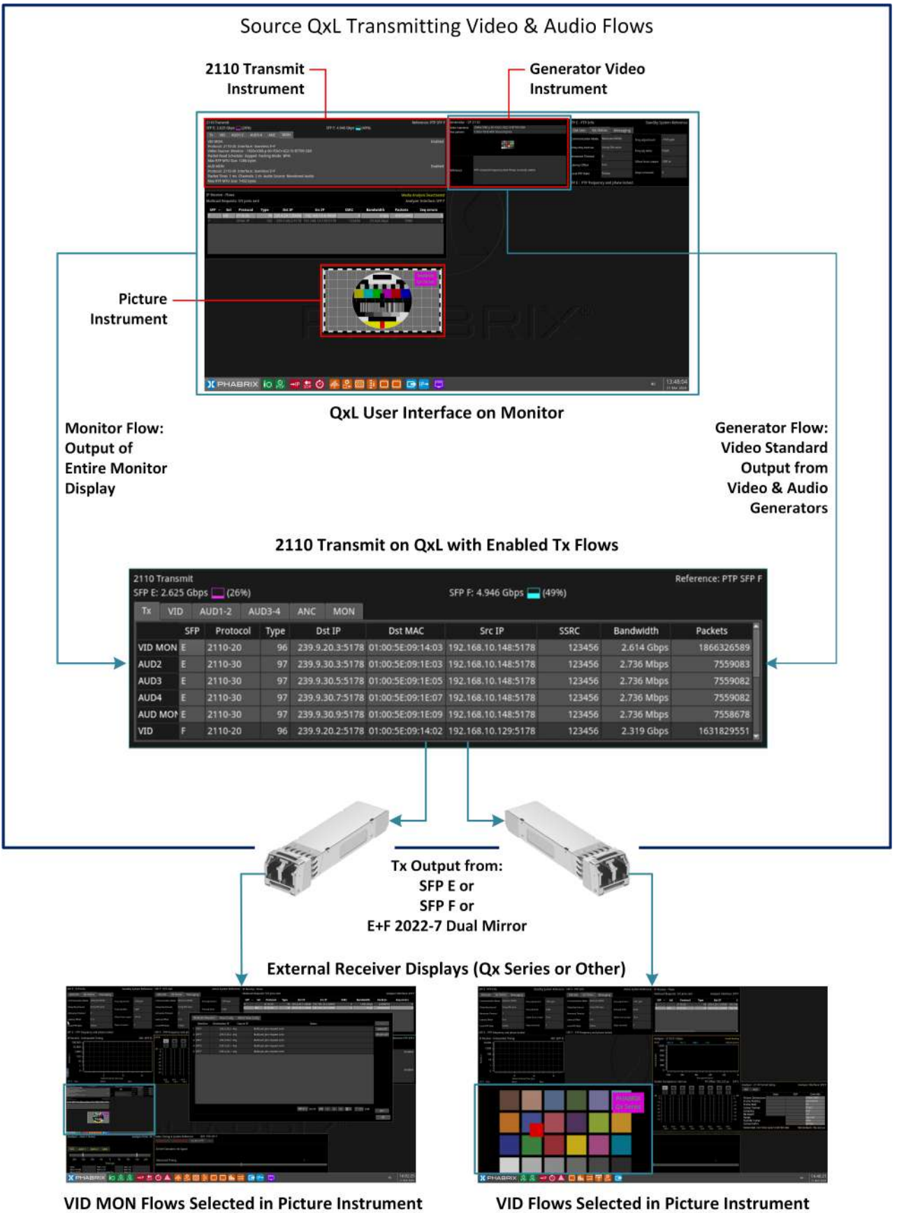
Figure 6-37: Schematic Overview of Transmission of Generator and Monitor Flows by the 2110 Transmit Instrument
