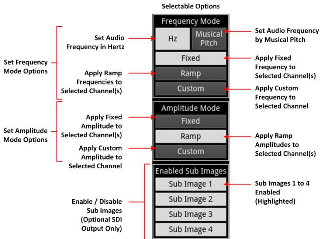
Figure 6-22: Audio Generator Configuration Dialog - Options Panel
