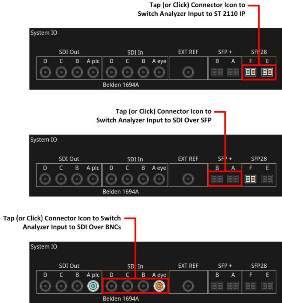
Figure 3-17: Confirmation Dialog to Switch Analyzer Input 1
