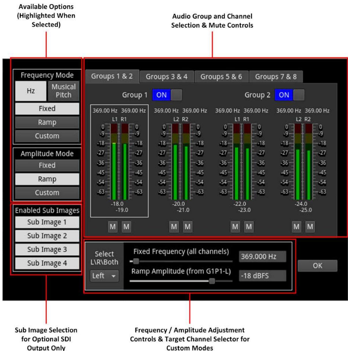
Figure 6-21: Generator Configuration - Audio Tab (ST 2022-6 IP and Optional SDI Output)
