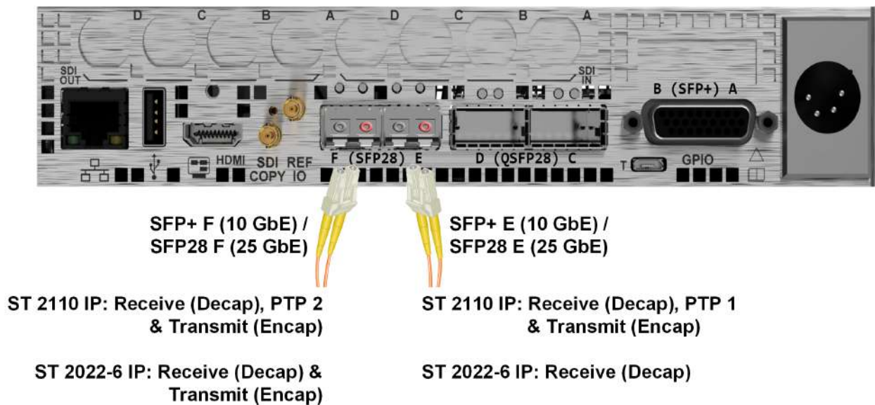
Figure 1-7: Connecting an IP-Only QxL (Option: PHQXL) Using SFP Connectors
