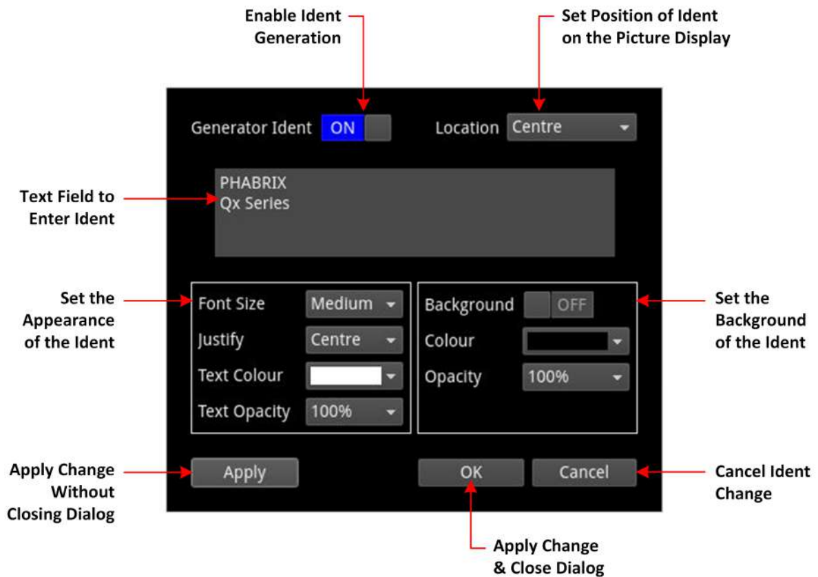
Figure 6-14: Generator - Generator Ident Dialog
