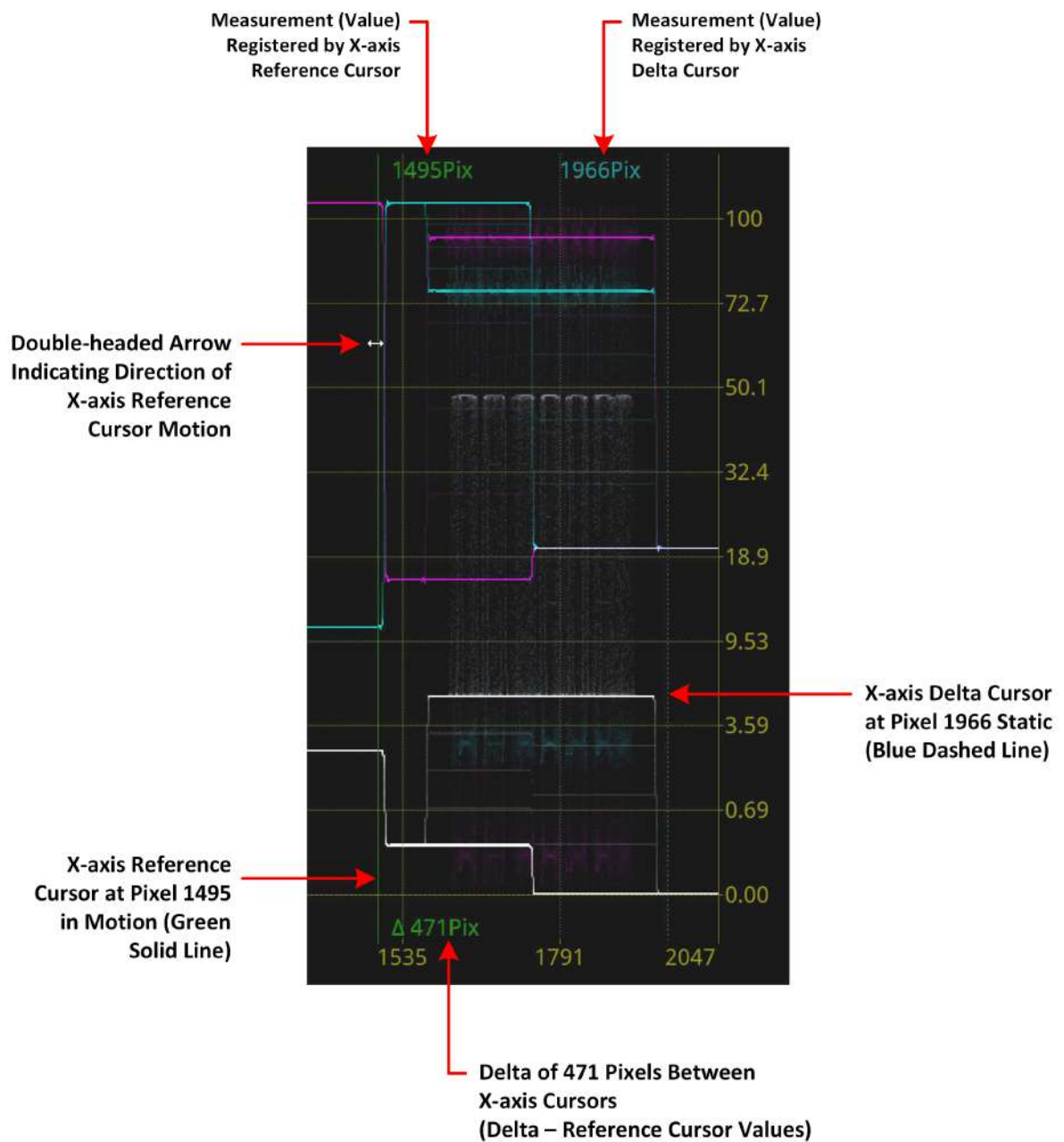
Figure 9-25: Waveform Measurement X-axis Cursors (Independent Configuration)
