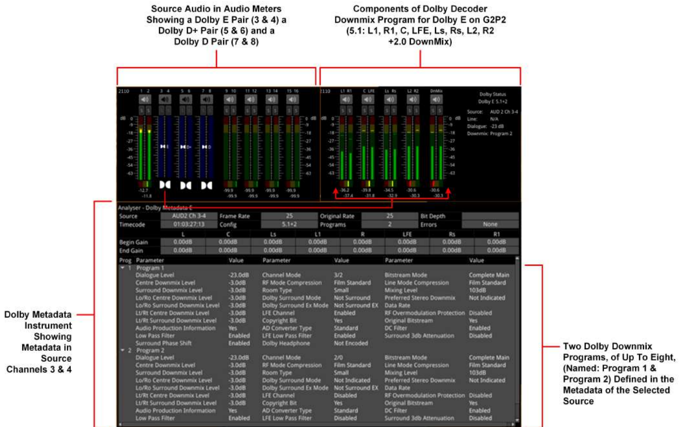
Figure 10-26: Audio Meters, Dolby Decoder and Dolby Metadata Instruments (ST 2110 Input)
