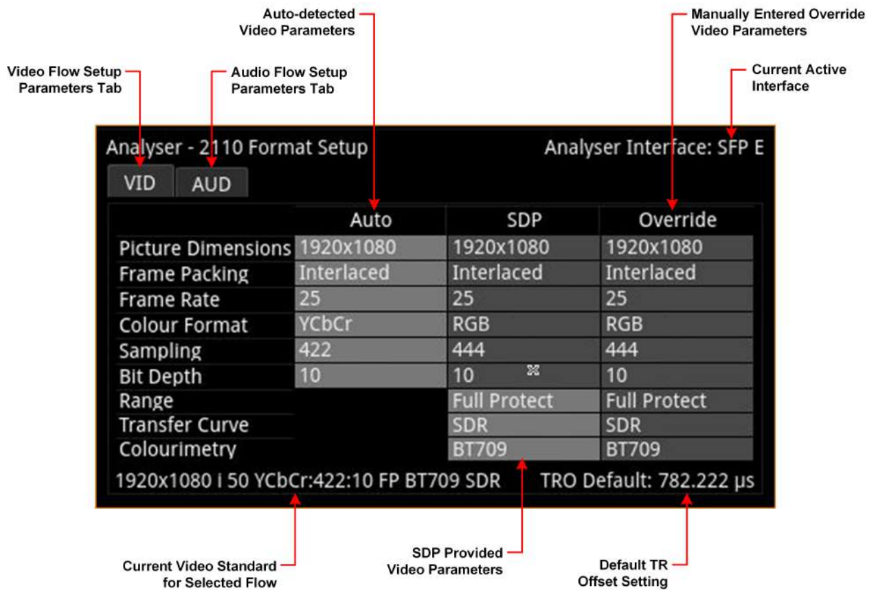
Figure 4-39: Analyzer - 2110 Format Setup Instrument - Video Tab
