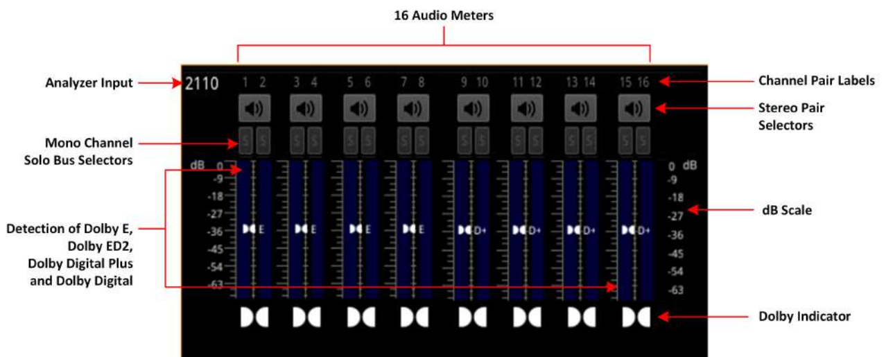
Figure 10-5: Analyzer - Audio Meters Instrument (ST 2110 IP Input)
