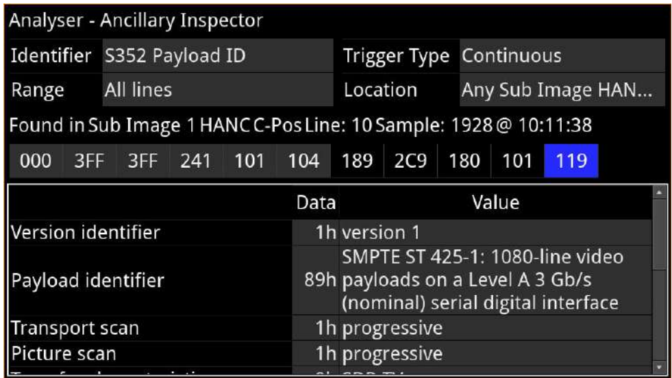
Figure 6-18: Analyzer - Ancillary Inspector Showing SMPTE ST352 Payload IDs
