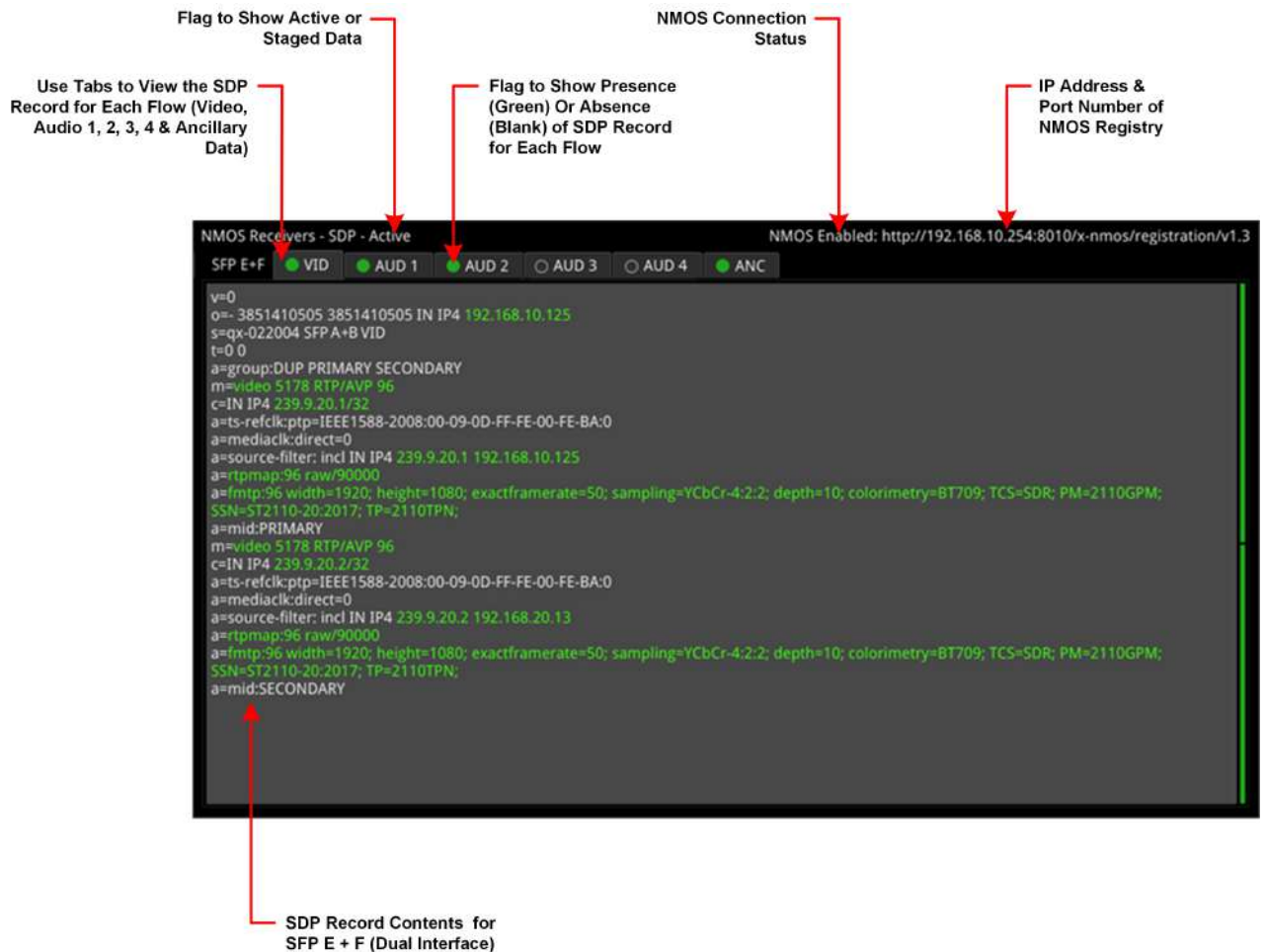
Figure 4-17: NMOS Receivers - SDP Instrument Views (Dual Interface, 1/4 Screen Size) (ST 2110 IP Input)
