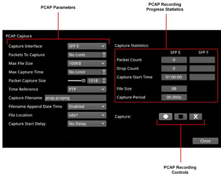
Figure 3-26: PCAP Capture Window
