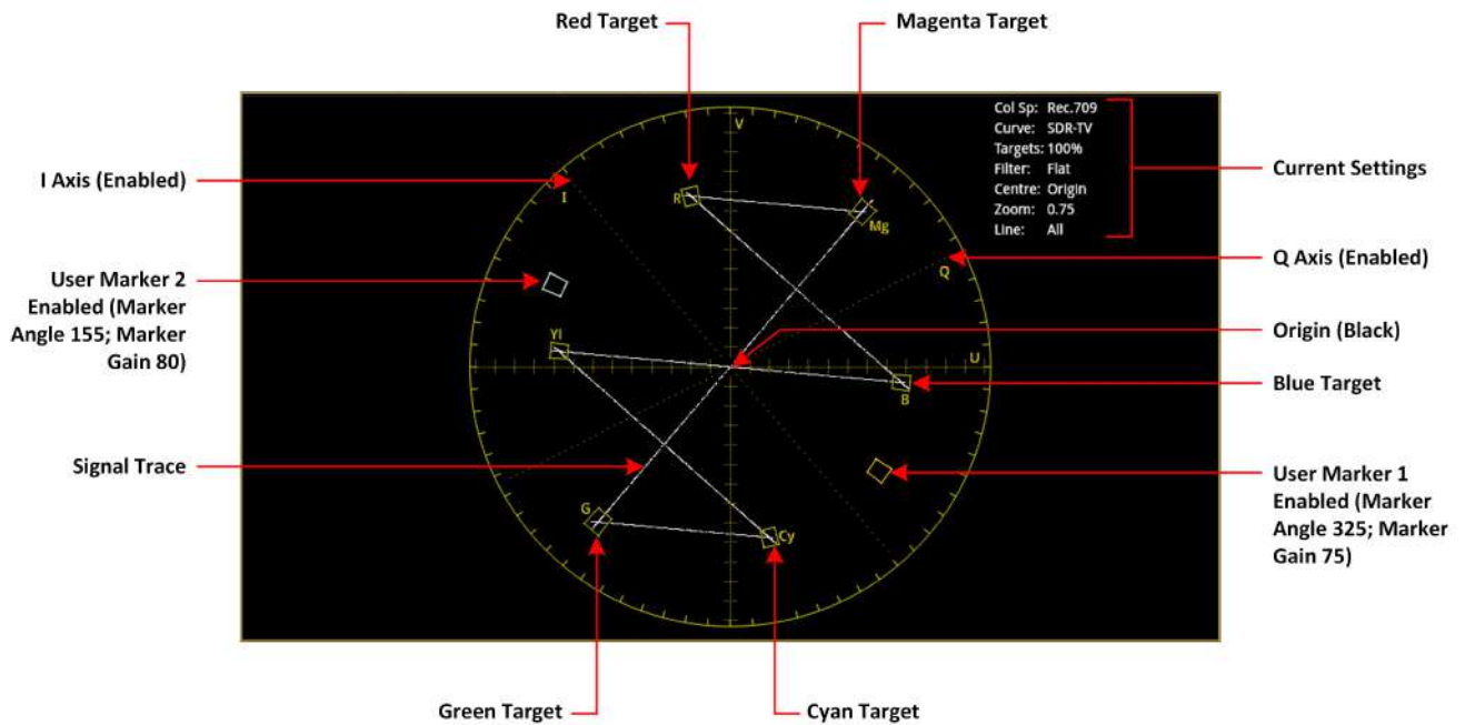
Figure 9-29: Analyzer - Vectorscope Instrument
