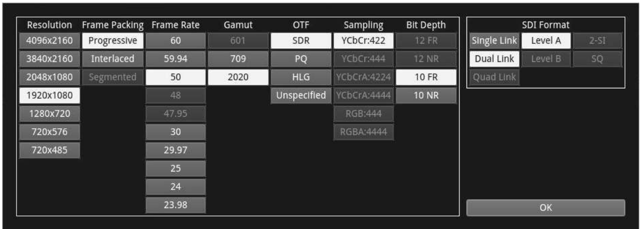
Figure 7-4: Analyzer - Video Standard Instrument - Manual Override Dialog (Optional SDI Input)
