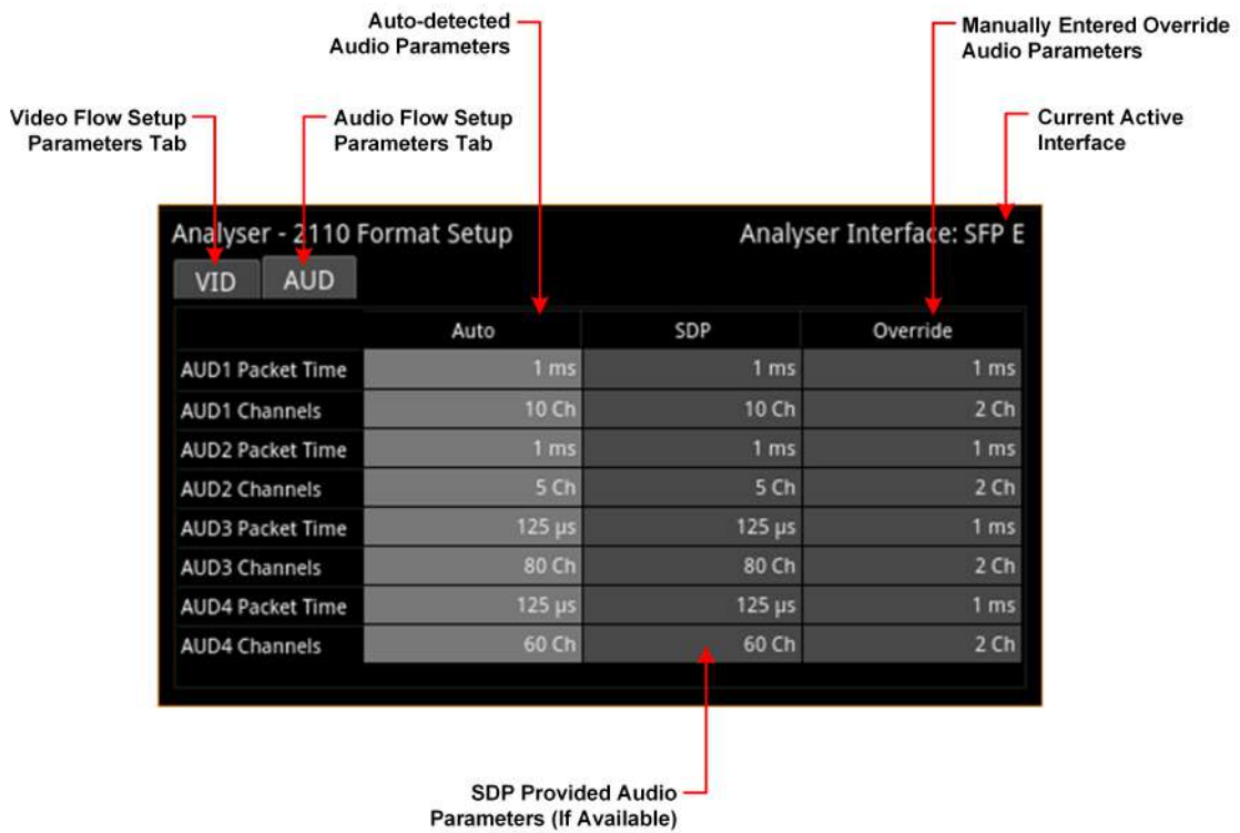
Figure 4-43: Analyzer - 2110 Format Setup Instrument - Audio Tab with Four Audio Flows
