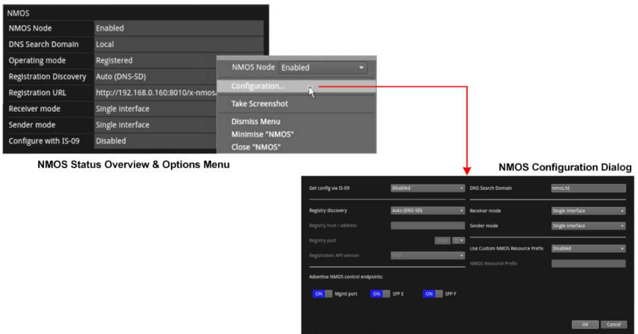
Figure 4-15: NMOS Instrument Options and Configuration Menu (ST 2110 IP Input)
