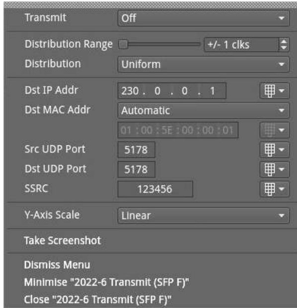
Figure 6-30: 2022-6 Transmit (SFP F) Menu Options
