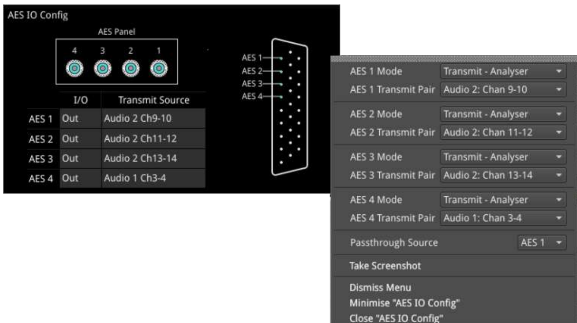
Figure 4-45: AES IO Config Instrument and Options Menu (ST 2110 IP Input)
