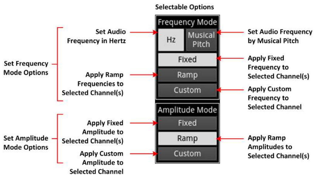
Figure 6-26: Audio Generator Configuration Dialog - Options Panel
