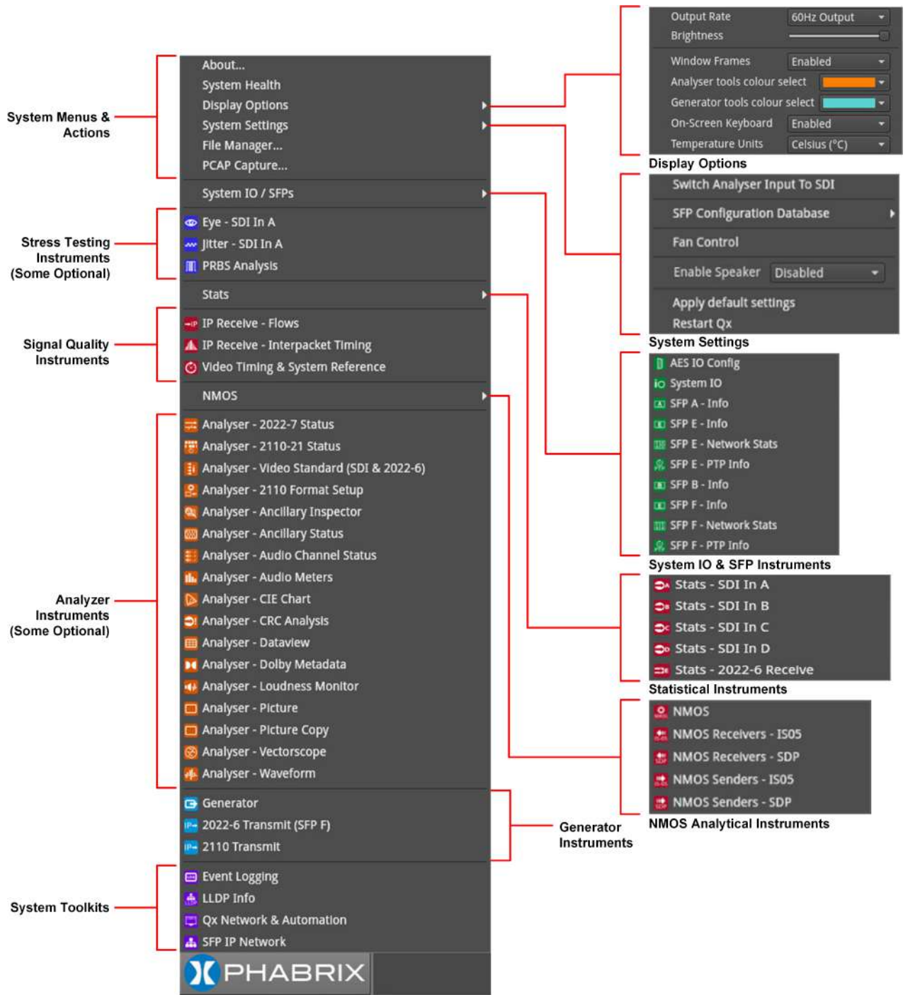
Figure 2-4: Launch Menu Showing Submenus
