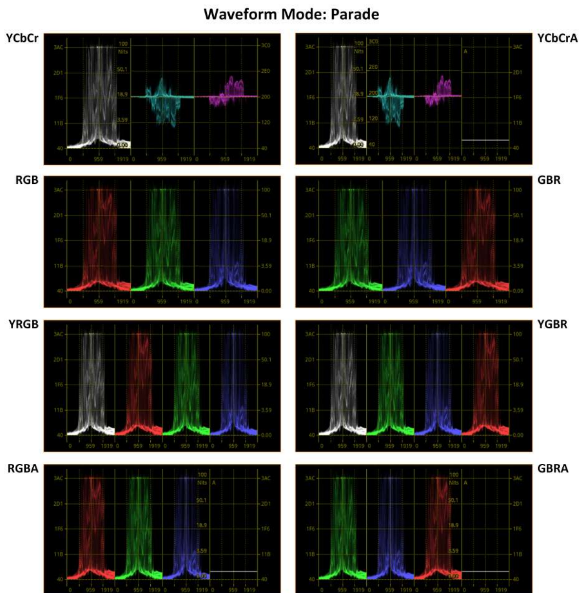
Figure 9-19: Parade Waveform Instrument Display Modes (Excludes Single Waveforms)
