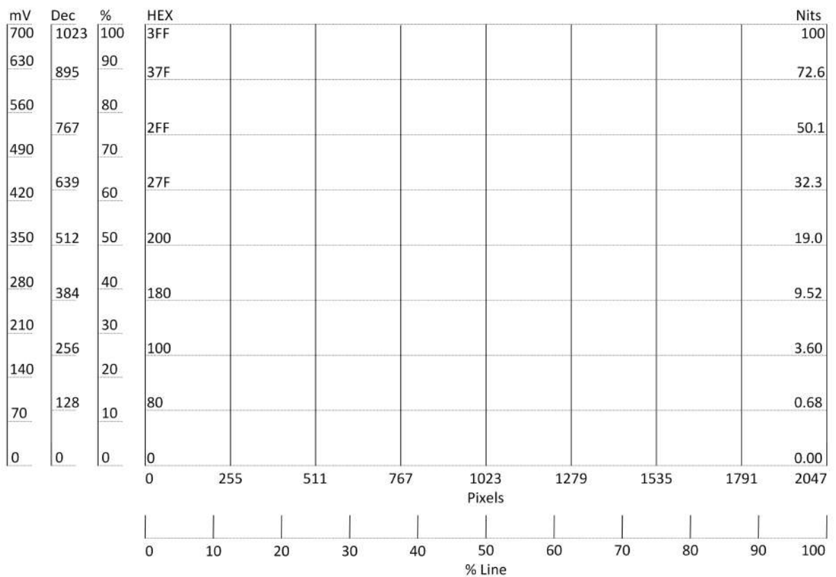
Figure 9-14: Schematic of Waveform Scales (Overlay Mode; SDR 2048 x 1080; Full Range, Full Screen Size)
