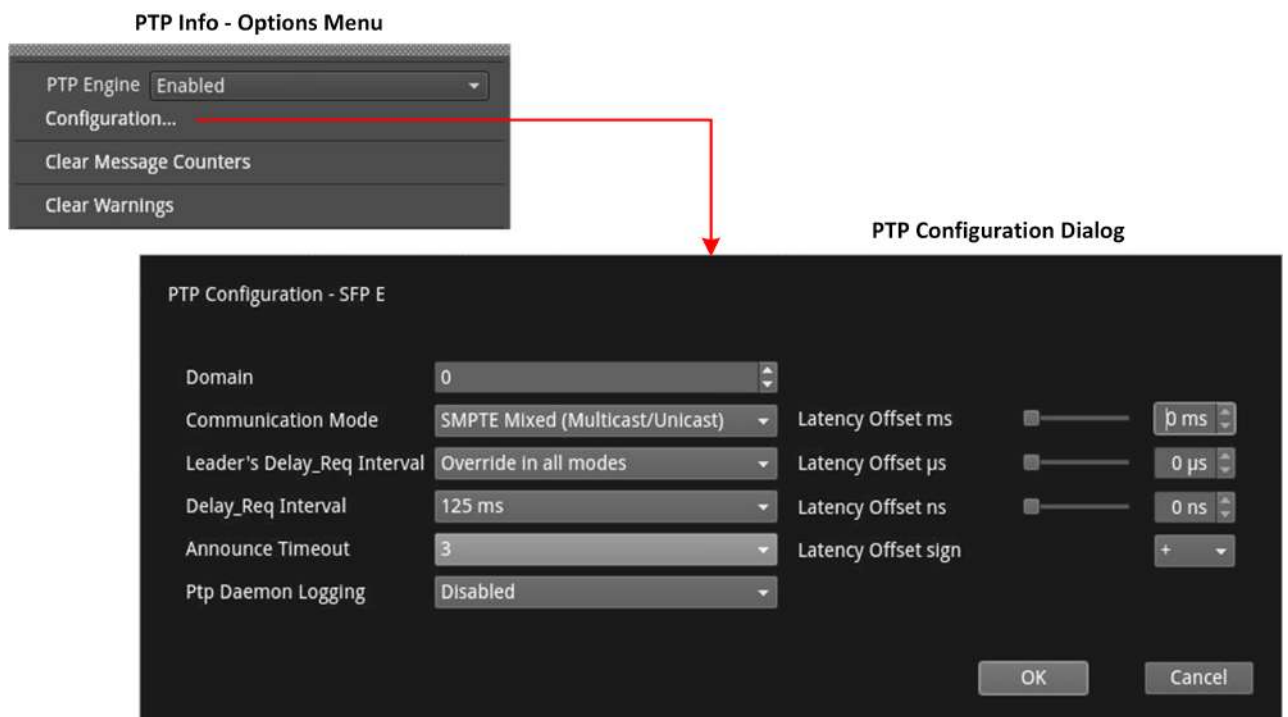
Figure 4-29: SFP E/F - PTP Info Instrument Menu Options
