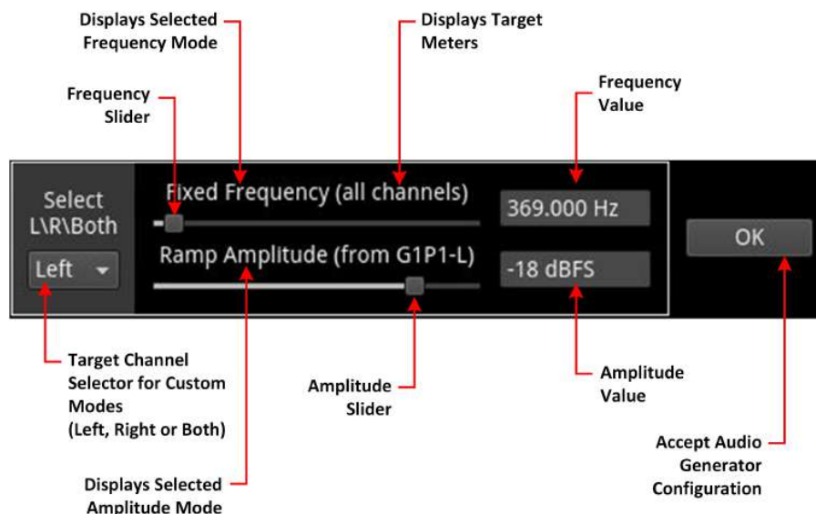
Figure 6-28: Audio Generator Configuration Dialog - Adjustment Controls
