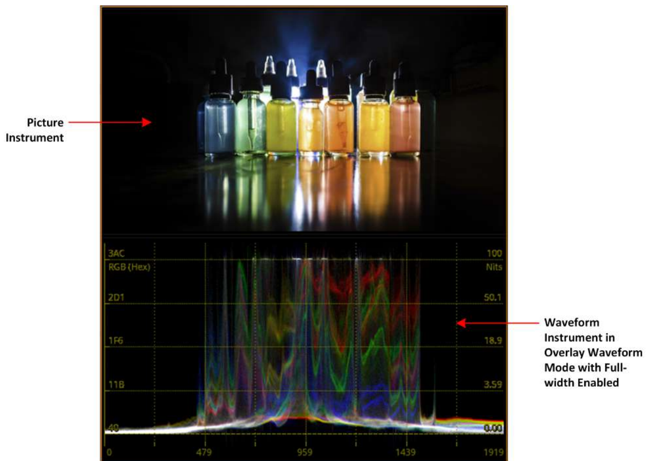
Figure 9-16: Waveform Instrument Matched to Width of Picture Instrument
