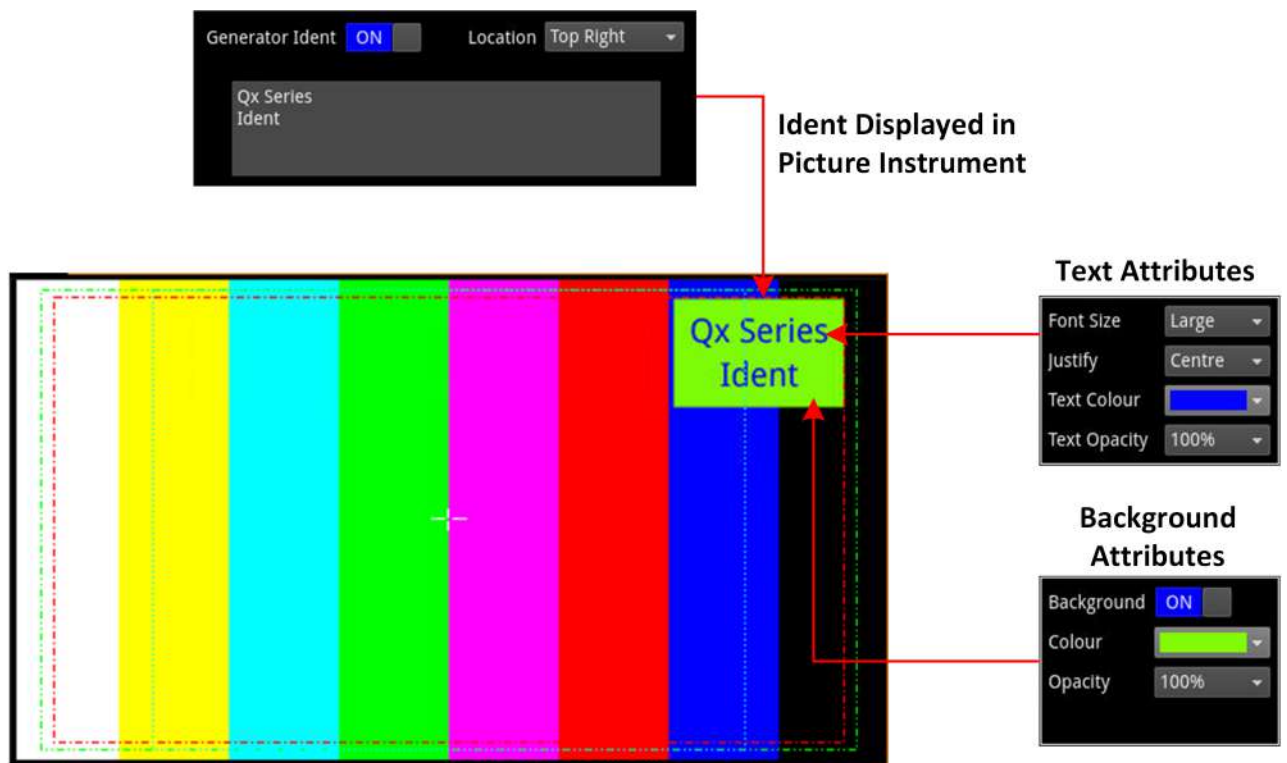
Figure 6-15: Generator Ident Displayed in Picture Instrument
