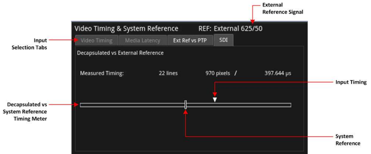
Figure 4-30: Video Timing & System Reference Instrument (ST 2022-6 IP Input)
