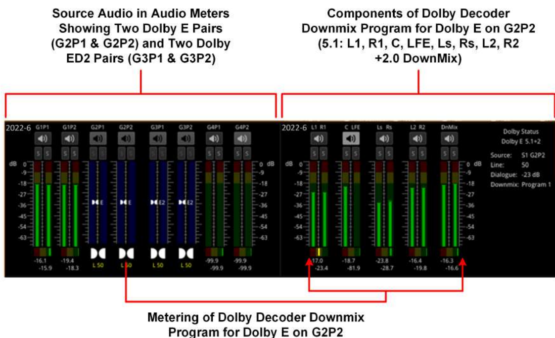
Figure 10-9: Audio Meters and Dolby Decoder Instruments (ST 2022-6 IP and Optional SDI Input)
