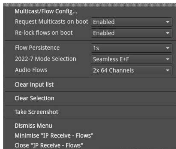
Figure 4-35: IP Receive - Flows Instrument Options Menu
