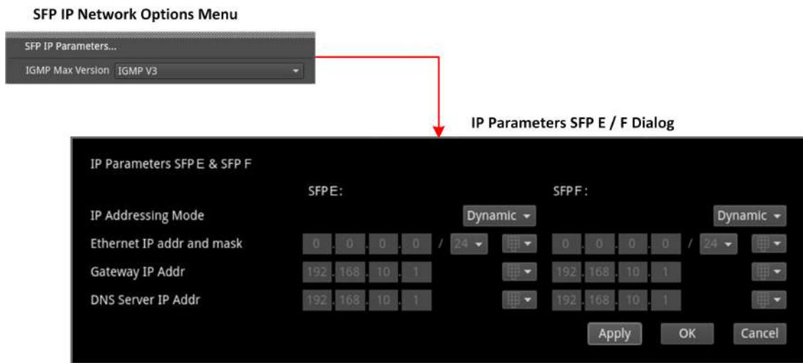
Figure 4-8: SFP IP Network Menu Options
