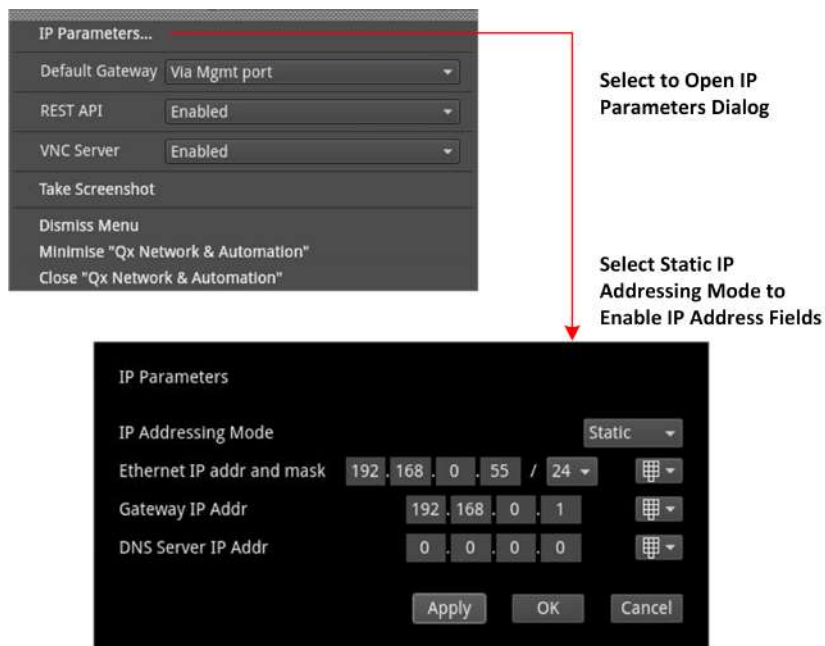
Figure 3-2: Qx Network & Automation Instrument Menu Options
