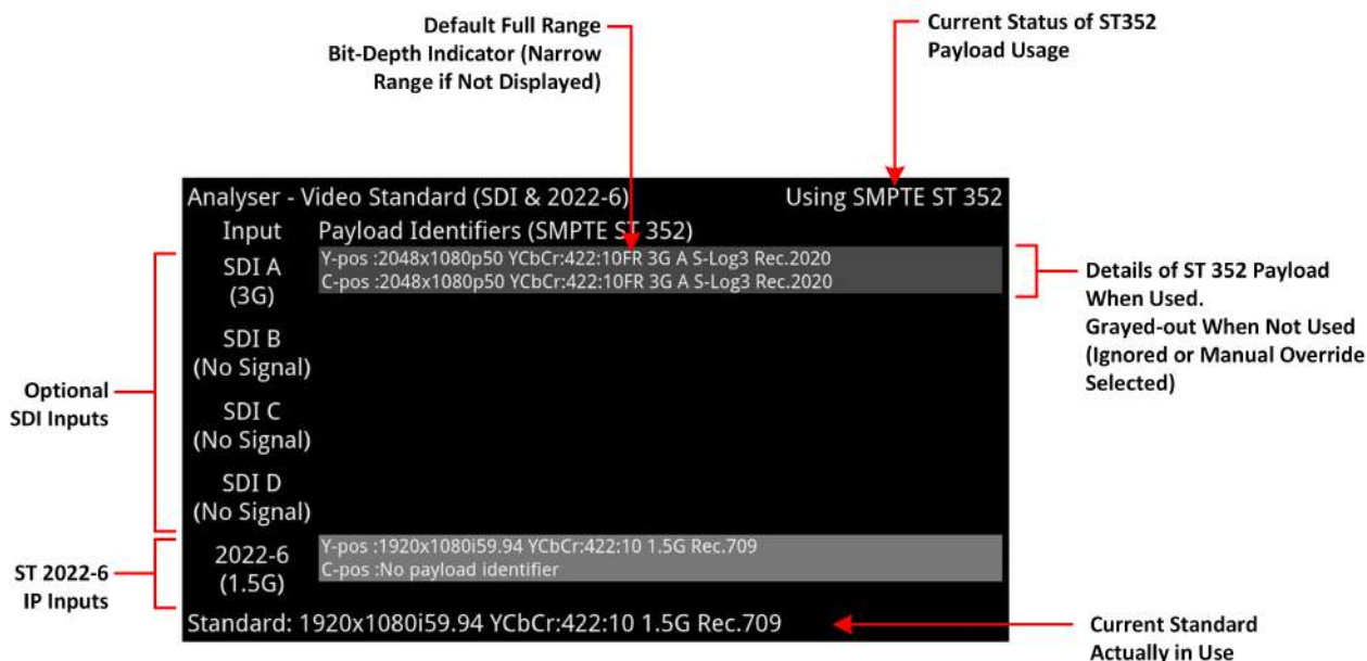
Figure 7-1: Analyzer - Video Standard (SDI & 2022-6) Instrument (Showing ST 2022-6 and Optional SDI Input)
