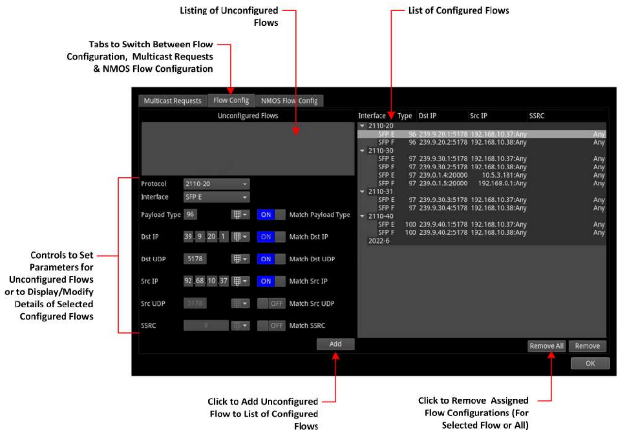
Figure 4-37: IP Receive - Flows: Flow Config Tab
