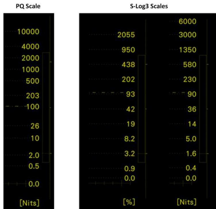
Figure 9-15: Comparison of PQ and S-Log3 Scales for HDR Waveform Analysis
