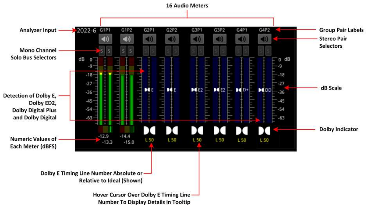
Figure 10-4: Analyzer - Audio Meters Instrument (ST 2022-6 IP and Optional SDI Input)
