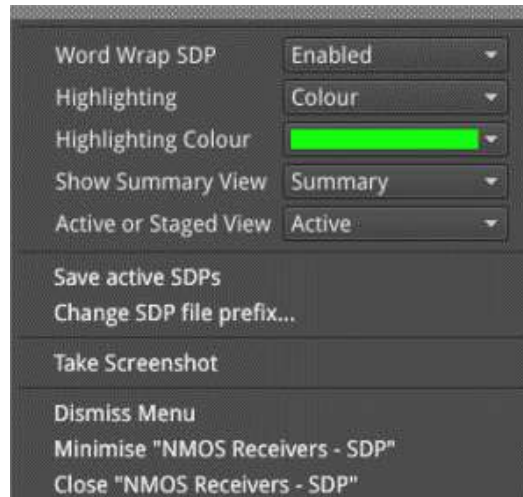
Figure 4-18: NMOS Receivers - SDP Instrument Menu Options
