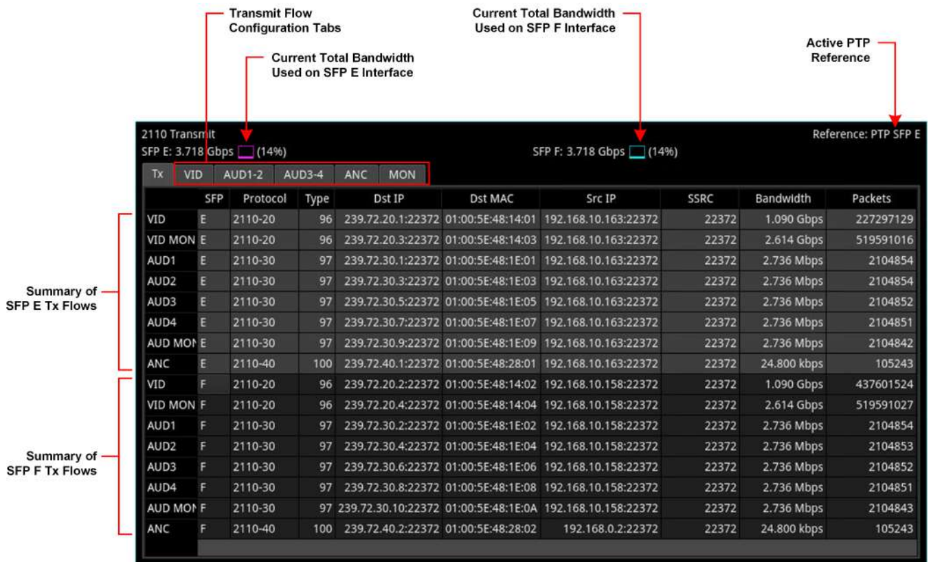
Figure 6-32: 2110 Transmit - Tx Tab
