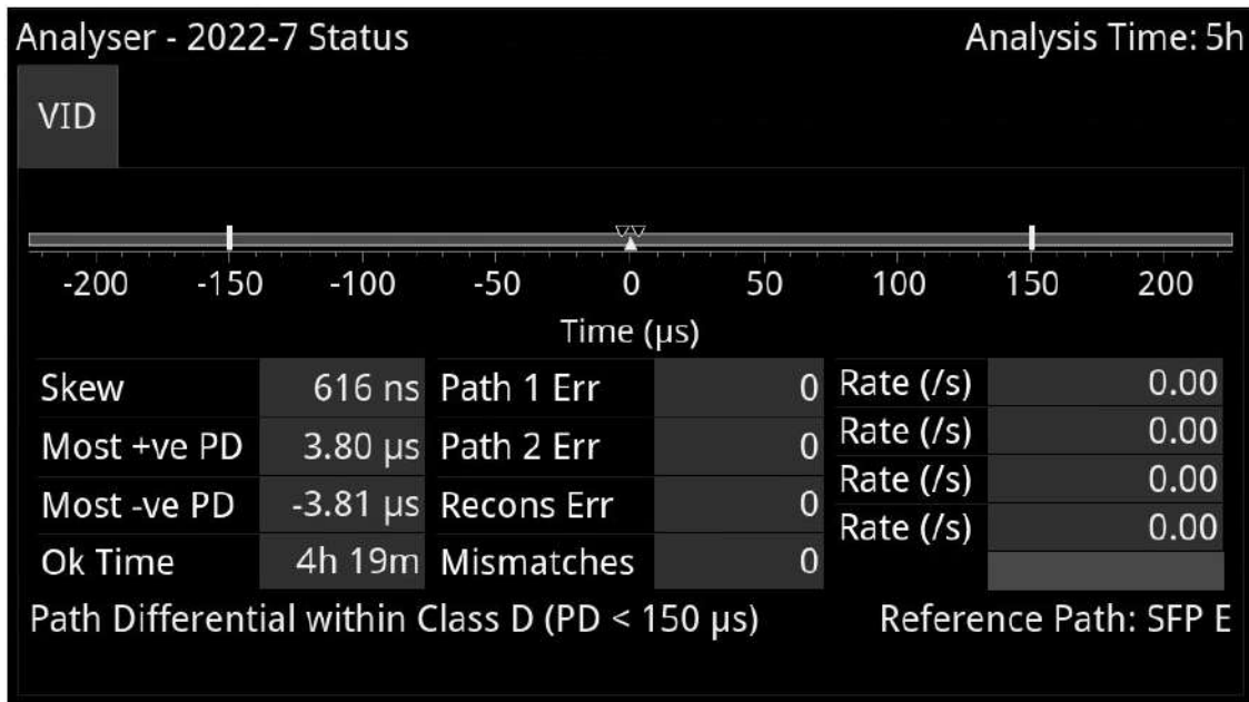
Figure 8-1: Analyzer - 2022-7 Status Instrument (ST 2022-6 IP Input)
